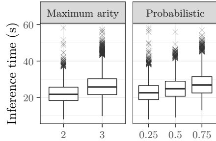
Fig. 4. Inference time for different values of \mathcal{M}_A and proportions of probabilistic facts that are probabilistic. The total number of facts is fixed at 10^5 .
